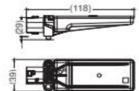
ASPÖCK TPMS SUB - RECEIVER ERX
