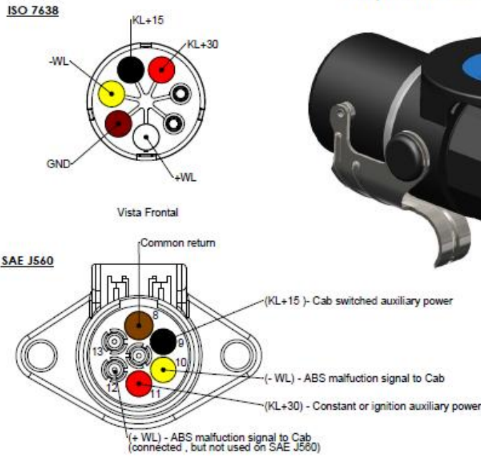
Adapter ISO 7638 to SAE J560 Auxiliary
